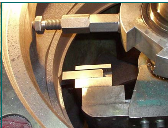
Machining cylinder liner seats on main engines
