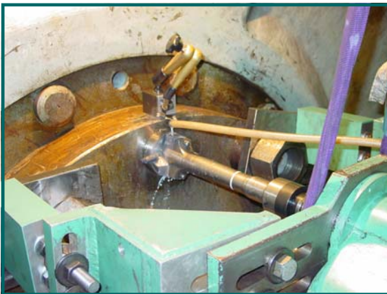
Boring fitting bolts of a flange-connection
